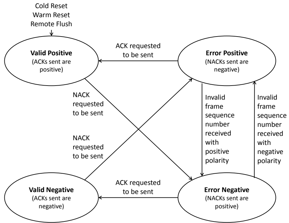
Figure 5-8 Receive Error State Machine
