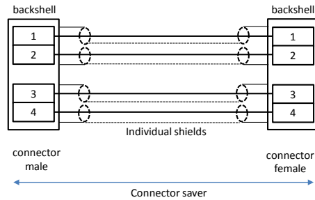
Figure 5-18 SpaceFibre flight connector saver
