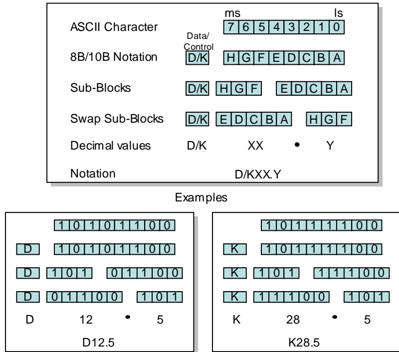
Figure A-3 8B/10B Notation
